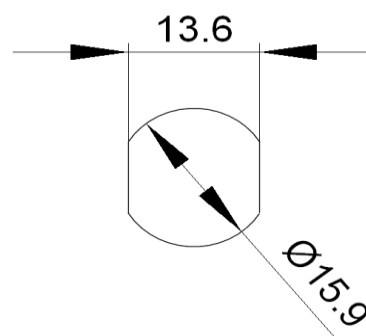
Panel cut dimensions
