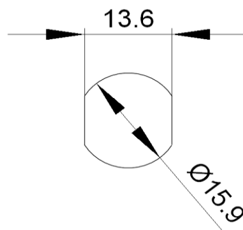
Panel cut dimensions
